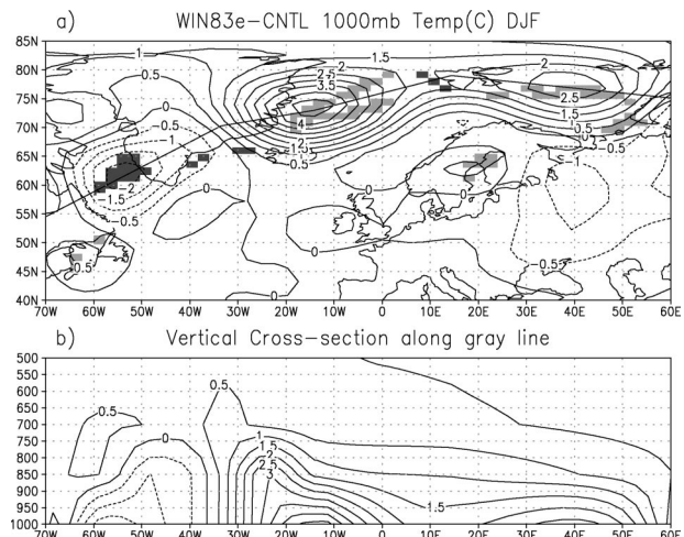
FIG. 4. Win83e temperature anomalies during DJF (a) at the 1000-mb level and (b) as a vertical cross section along the transect line shown in (a) (contours have an interval of 0.5^\circ\text{C} ; negative contours dashed). As in Fig. 2, the light (dark) shading indicates grid squares with less (more) ice in Win83e than in Cntle during Jan 1983.
