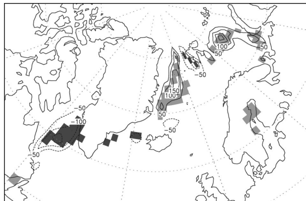
FIG. 3. Win83e net upward heat flux anomalies over the North Atlantic during DJF of 1982/83 (contours have an interval of 50 \text{ W m}^{-2} ; negative values dashed, zero contour omitted). The anomalies are defined as the ensemble mean of the 50 Win83e simulations minus the long-term mean of the 55-yr control (Cntle) integration. The light (dark) shading indicates grid squares with less (more) ice in Win83e than in Cntle during Jan 1983; only one month is shown because it is unclear how to average a binary quantity like ice extent when it varies over a season.
