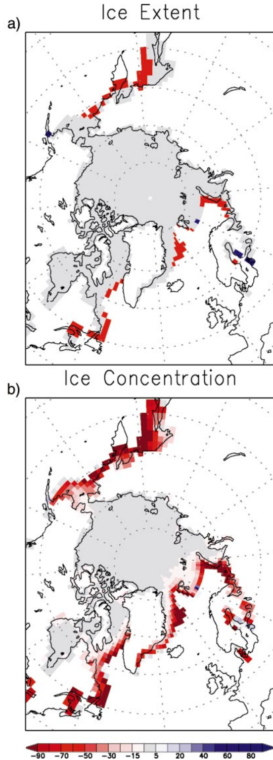
FIG. 14. Sea ice boundary conditions during Jan 1996 in the Win96 (a) extent and (b) concentration experiments. Gray indicates areas with climatological sea ice, blue (red) indicates grid squares with increased (reduced) ice relative to the climatology. The percent change in ice cover in Win96c relative to the Cntle simulation is given by the scale beneath (b).
