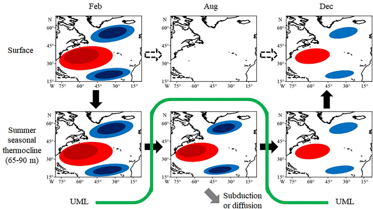
Fig. 8 Schematic representation of the SSTA tripole reemergence process in the North Atlantic ( 15^{\circ} – 70^{\circ} N 8^{\circ} – 80^{\circ} W). Positive and negative temperature anomalies (related to the NAO positive phase; for the NAO negative phase, the signs of the anomalies are opposite) associated with the tripole pattern are represented by the red and blue ovals. The size of the ovals determines the area of the anomalies, and the color determines their amplitude (dark red (dark blue) cor-
