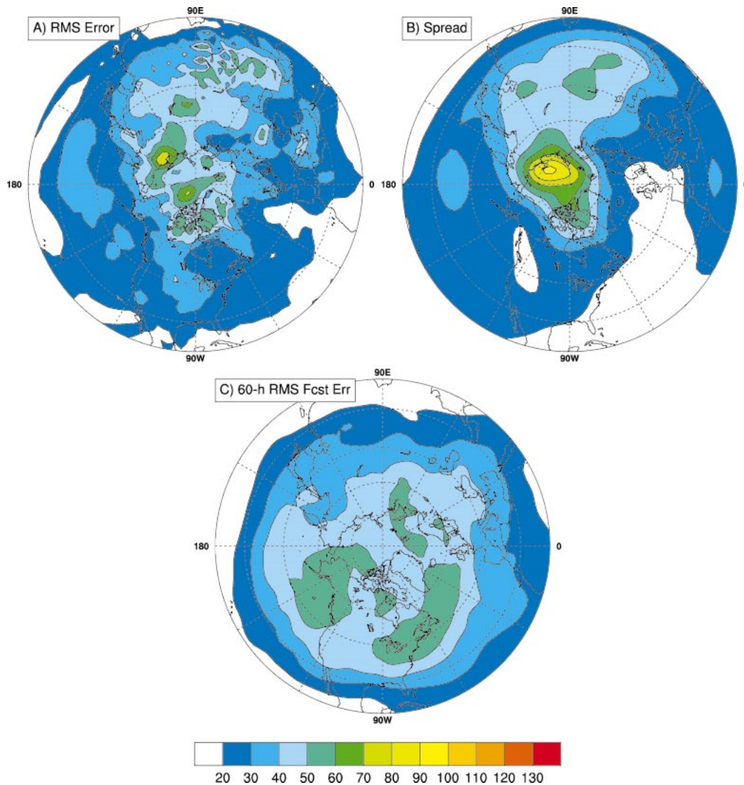
FIG. 4. Maps of 500-hPa geopotential height (a) ensemble mean analysis error, and (b) ensemble spread averaged over the 124 Dec analyses for the simulated 1915 surface pressure network. (c) Mean 60-h 500-hPa geopotential height forecast error for forecasts initialized from all 744 0000 UTC Dec NCEP–NCAR reanalyses for 1979–2002. Units are in meters.
