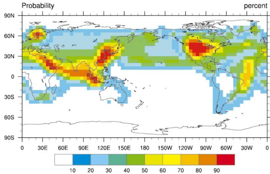
FIG. 2. Map of probabilities used to create simulated 1915 surface pressure network. Probabilities represent the average number of daily historical surface pressure observations in each 5^\circ box normalized by the average number of daily surface pressure observations in the reduced 2001 network. See text for details.
