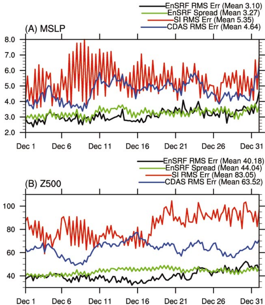
FIG. 3. Time series of rms analysis error and ensemble spread averaged over the Northern Hemisphere poleward of 20^{\circ}\text{N} for (a) mean sea level pressure (hPa) and (b) 500-hPa geopotential height (m).
