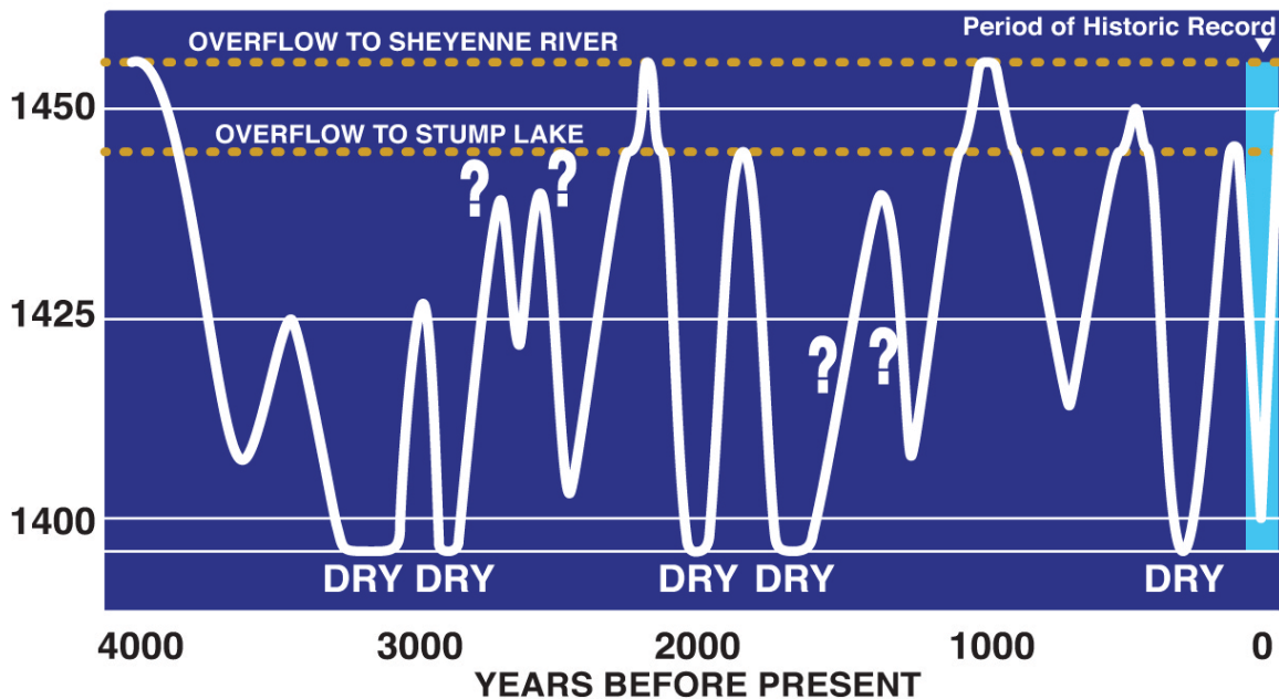
Figure 1. Devils Lake water levels based on paleoecological studies of sediment deposits in the lake bed (Bluemlle, 1991; Murphy et al., 1997). Low (high) water levels are inferred to correspond to dry (wet) climate conditions. Direct measurements have been taken during the period shown in light blue. The current strong centennial rise in water levels detected by gage measurements is commensurate with historical fluctuations. Graphics Source: North Dakota State Water Commission Fact Sheet, available at http://swc.state.nd.us/4dlink9/4dcgi/GetContentPDF/PB-206/DLFactSheet2010.pdf
