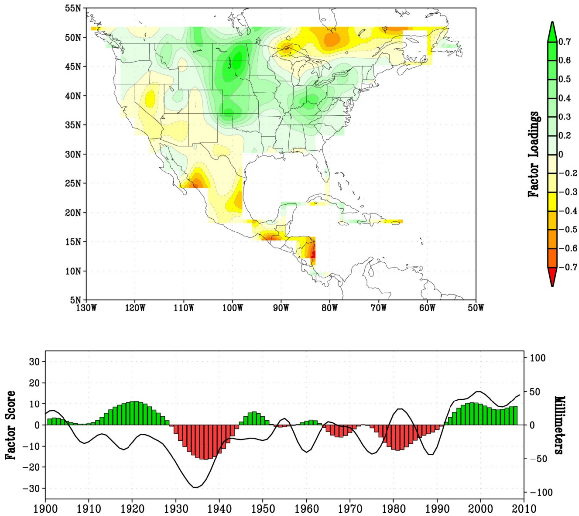
Figure 8. The statistical pattern of observed annual precipitation variability using the method of Empirical Orthogonal Function (EOF) analysis. The spatial plot shows the fourth leading pattern of precipitation variability for North America as a whole. This pattern is shown because it is one of two dominant national patterns, with strong amplitude over the Great Plains region. The time series of this empirical pattern is shown in the lower panel. The superimposed black contour is the smoothed annual precipitation time series averaged over Devils Lake. PPT denotes precipitation. Data available at http://www.esrl.noaa.gov/psd/data/gridded/data.gpc.html .
