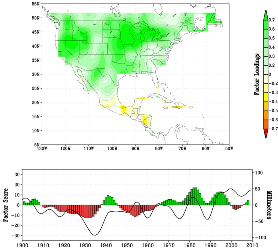
Figure 7. The statistical pattern of observed annual precipitation variability using the method of Empirical Orthogonal Function (EOF) analysis. The spatial plot shows the second leading pattern of precipitation variability for North America as a whole. This pattern is shown because it is one of two dominant national patterns, with strong amplitude over the Great Plains region. The time series of this empirical pattern is shown in the lower panel. The superimposed black contour is the smoothed annual precipitation time series averaged over Devils Lake. PPT denotes precipitation. Data available at http://www.esrl.noaa.gov/psd/data/gridded/data.gpcp.html .
