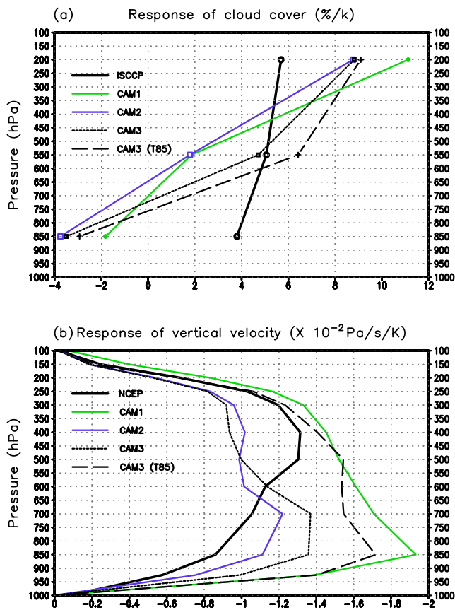
Figure 8. Responses of (a) cloud cover from ISCCP observations and four models and (b) vertical velocity from the NCEP reanalysis and four models to El Niño warming as a function of height averaged over the equatorial Pacific ( 160^{\circ}\text{E} – 290^{\circ}\text{E} , 5^{\circ}\text{S} – 5^{\circ}\text{N} ). The cloud cover data used here are the high, middle and low cloud cover (indicated by the markers shown in Figure 8a) for both models and observations, the same as those used by Sun et al. [2003] and Zhang and Sun [2006]. Shown in every vertical level are regression coefficients obtained by linearly regressing the concerned quantities at the corresponding level against the underlying SST averaged over the region of El Niño warming ( 160^{\circ}\text{E} – 290^{\circ}\text{E} , 5^{\circ}\text{S} – 5^{\circ}\text{N} ). The interannual variations of the concerned quantities over the ERBE period are used for the regression calculations.
