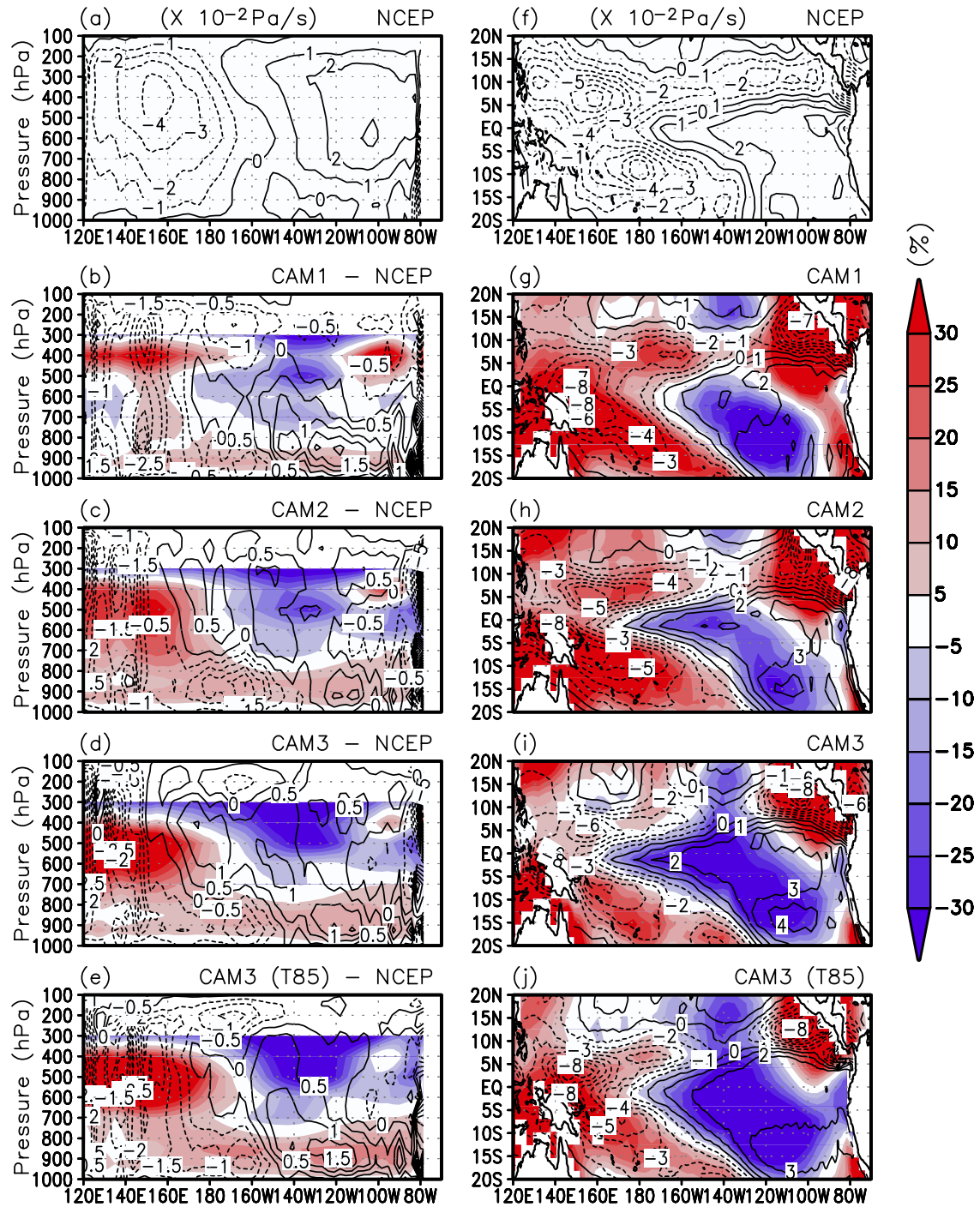
Figure 4. Vertical cross sections of (a–e) annual mean vertical velocity averaged over the equator (5°S–5°N) from NCEP data and the difference between models and NCEP data and (f–j) spatial patterns at 400 hPa for annual mean vertical velocity from NCEP reanalysis and four models over the ERBE period. The shaded values in Figures 4b–4e and 4g–4j are the percentage differences in annual mean specific humidity between the models and NCEP data over the same period. They are obtained from the differences between models and NCEP data divided by the values of NCEP data.
