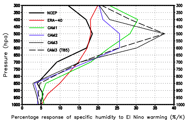
Figure 2. Percentage response of specific humidity to El Niño warming as a function of height from the NCEP-NCAR reanalysis, ERA-40 reanalysis, and four models averaged over the equatorial Pacific (160–290°E, 5°S–5°N). Shown are regression coefficients divided by the respective climatology. In every vertical level, the regression coefficients are obtained by linearly regressing specific humidity at the corresponding level against the underlying SST (as given by Zhang and Sun [2006, Figure 19]) averaged over the region of El Niño warming (160–290°E, 5°S–5°N). The interannual variations of specific humidity over the ERBE period are used for the regression calculations.
