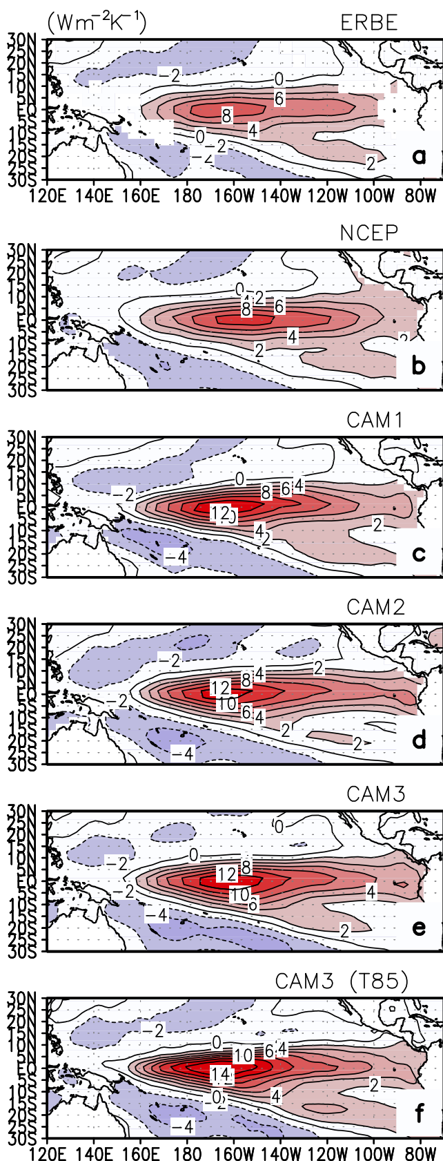
Figure 1. Response of the clear-sky greenhouse effect to El Niño warming from (a) ERBE observations, (b) NCEP reanalysis, (c) CAM1, (d) CAM2, (e) T42 CAM3, and (f) T85 CAM3. Shown are regression coefficients obtained by linearly regressing the clear-sky greenhouse effect at each grid point against the underlying SST averaged over the region of El Niño warming ( 160^{\circ}\text{E} – 290^{\circ}\text{E} , 5^{\circ}\text{S} – 5^{\circ}\text{N} ). The interannual variations of greenhouse effect over the ERBE period are used for the calculations.
