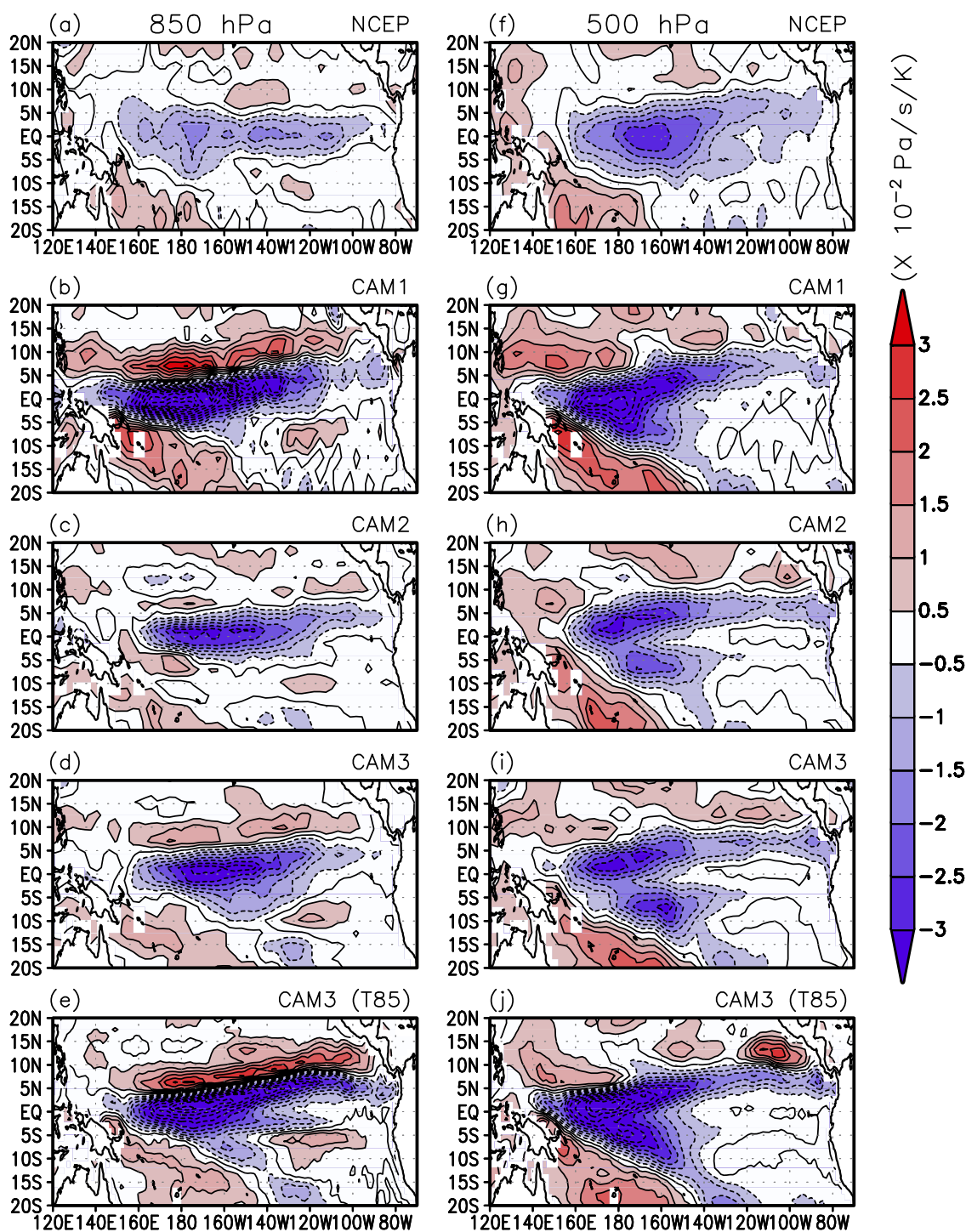
Figure 5. Spatial pattern of the response of vertical velocity to El Niño warming (a–e) at 850 hPa and (f–j) at 500 hPa from the NCEP-NCAR reanalysis and four models. Shown are regression coefficients obtained by linearly regressing vertical velocity against the underlying SST averaged over the region of El Niño warming (160–290°E, 5°S–5°N). The interannual variations of vertical velocity over the ERBE period are used for the regression calculations.
