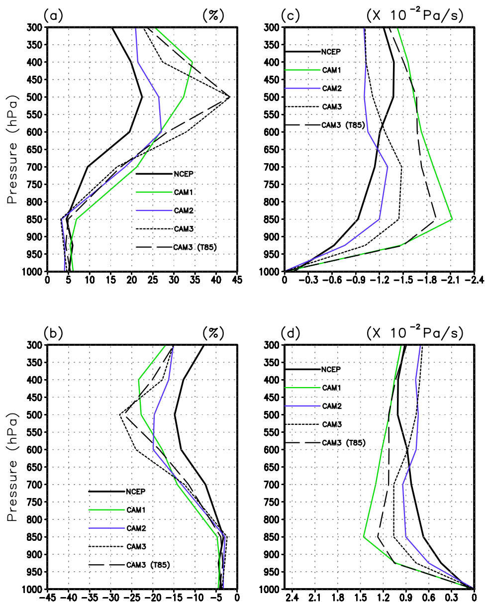
Figure 7. Composite percentage changes in specific humidity during (a) warm periods and (b) cold periods as a function of height from the NCEP-NCAR reanalysis and four models averaged over the equatorial Pacific ( 160\text{--}290^\circ\text{E} , 5^\circ\text{S}\text{--}5^\circ\text{N} ). The percentage changes in specific humidity are calculated as the anomalies divided by the respective climatology. Also shown are the composite changes in vertical velocity during (c) warm periods and (d) cold periods as a function of height from the NCEP-NCAR reanalysis and four models averaged over the equatorial Pacific ( 160\text{--}290^\circ\text{E} , 5^\circ\text{S}\text{--}5^\circ\text{N} ). The warm and cold periods are defined as the periods when the Niño-3 SST anomalies are larger than 0.3^\circ\text{C} and less than -0.3^\circ\text{C} over the ERBE period, respectively.
