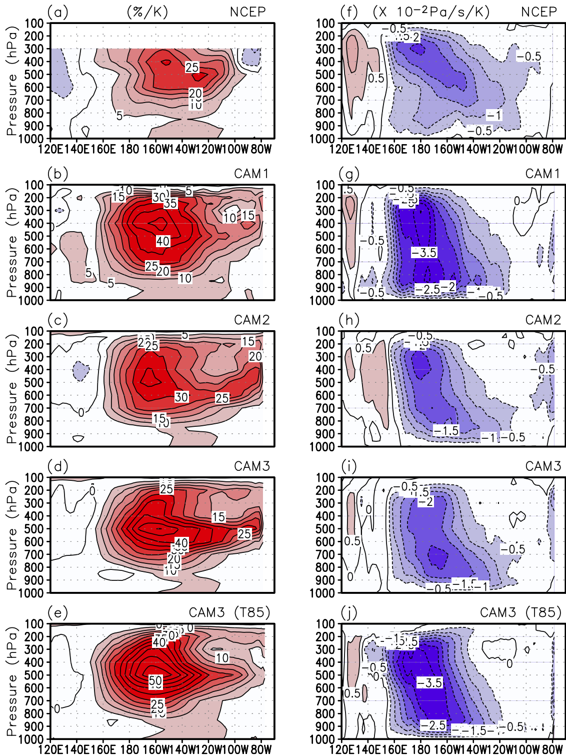
Figure 6. Vertical cross sections averaged over the equator ( 5^{\circ}\text{S} – 5^{\circ}\text{N} ) for (a–e) the percentage response of specific humidity and (f–j) the response of vertical velocity to El Niño warming from NCEP data and four models. Shown in every vertical level are the responses obtained by the same way as in Figures 2 and 5.
