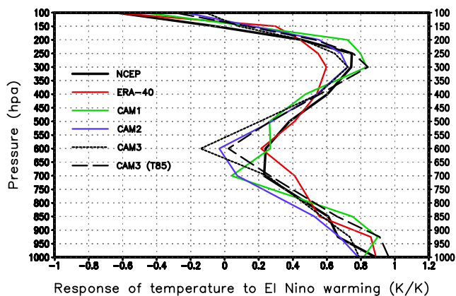
Figure 3. Response of air temperature to El Niño warming as a function of height from the NCEP-NCAR reanalysis, ERA-40 reanalysis, and four models averaged over the equatorial Pacific (160–290°E, 5°S–5°N). Shown in every vertical level are regression coefficients obtained by linearly regressing the air temperature at the corresponding level against the underlying SST averaged over the region of El Niño warming (160–290°E, 5°S–5°N). The interannual variations of air temperature over the ERBE period are used for the regression calculations.
