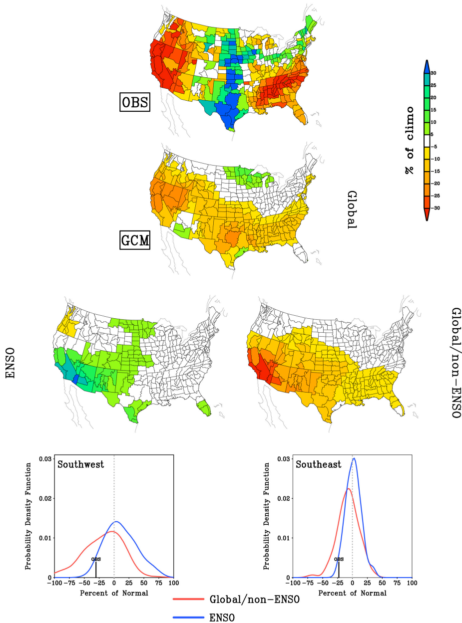
Fig. 1. The U.S. 2007 annually averaged (January-December) precipitation departures expressed as % of the 1971-2000 climatologies for observations (top), for simulations based on global SST forcing (middle, contour interval half as for OBS), for simulations based on tropical east Pacific SST forcing (bottom left, same contour interval as for OBS), and for simulations based on global SST forcing excluding the tropical east Pacific (global/non-ENSO; bottom right, same contour interval as for OBS). The probability distribution functions of regional precipitation departures of the individual 150-member runs for the ENSO forced (blue curve) and global/non-ENSO forced regions (red curve) are shown for the Southwest U.S. (left) and the Southeast U.S. (right). Observed 2007 annual precipitation departures are shown by vertical gray bar.
