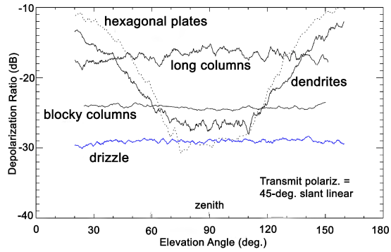
Figure 2. Particle type DR signatures from RHI scans with the NOAA/K radar (Reinking et al. 2000).
