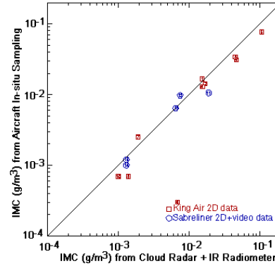
Figure 3. Ice mass content in a cirrus cloud estimated from NOAA/K radar and IR radiometer measurements and from aircraft in-situ samples (Matrosov et al. 1998).
